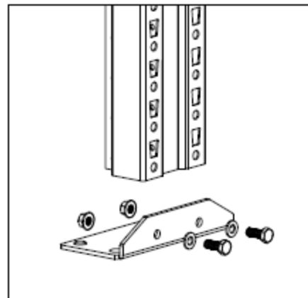
upright – base plate bolted connection
